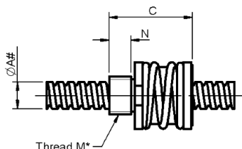
Part number selection table - LCMY series, thread mount
