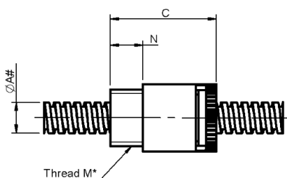
Part number selection table - LNTGY series, thread mount
