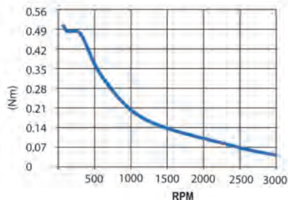
RCM1_-17L30-E-RT3
