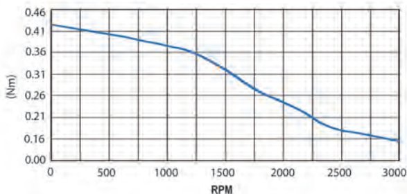
RCM1-_-23S30-C-RT3
