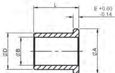
Flanged
