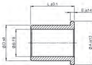
Flanged
