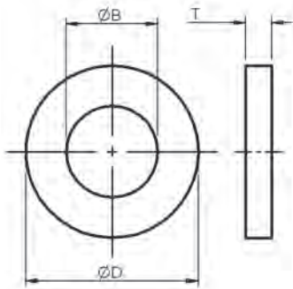
Plain Washers
