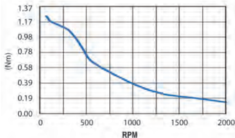
RCM1- -23L20-E-RT3
