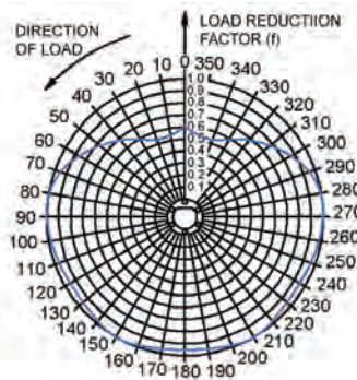
Closed bearing 6 rows of balls
